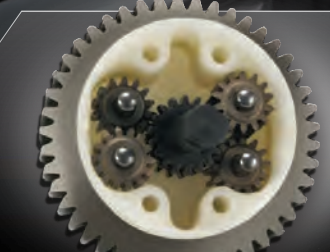
Planetary Differential
